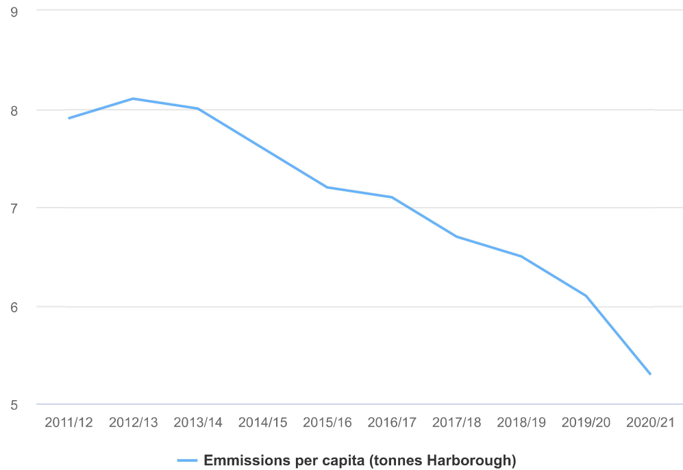
CLIM EAP 03 Per Capita Emissions CO2 Harborough (tonnes)
